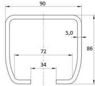
Cantilever Track /HDG/ Parameters in mm (millimeters)
